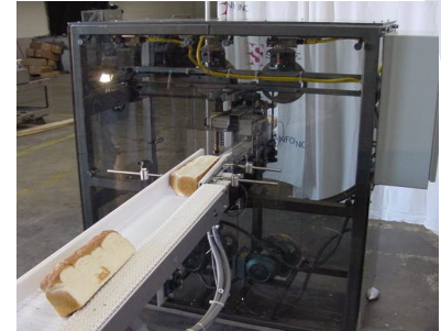
Tipping Conveyor
