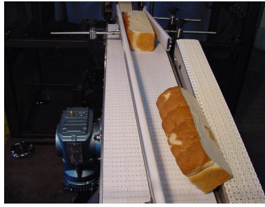
Tipping Conveyor
